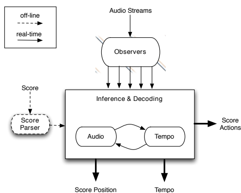
Figure 1. General Design Diagram of Antescofo
