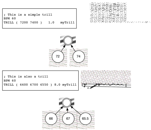
Figure 4. Antescofo 's score sample and state transition diagram for TRILL class
